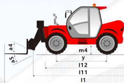
Machine on tyres with forks - with levelling device Metric
